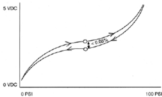
Figure 2: Hysteresis Graph
