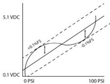
Best Fit Straight Line Method (BFSL)
