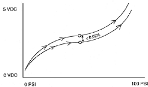
Figure 3: Repeatability Graph
